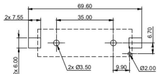
PCB MOUNTING LAYOUT
