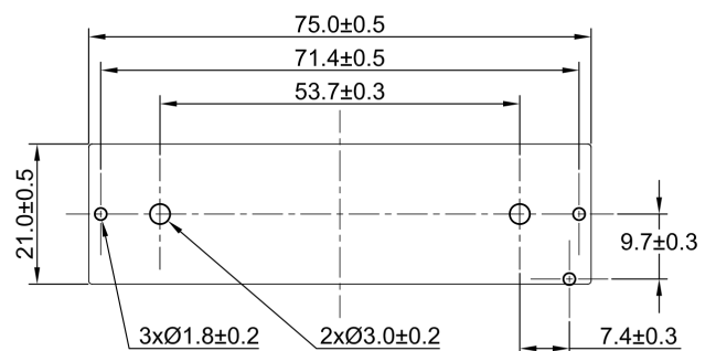
PCB/MOUNTING LAYOUT
