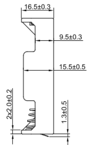
BH-381-3B Shown With Snap Terminals
