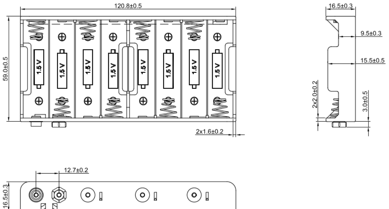
BH-381-3B Shown With Snap Terminals
