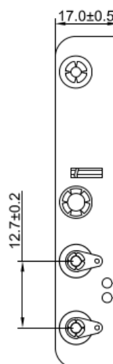
BH-351B Shown without Snap Terminals
