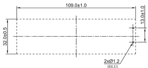
PCB/MOUNTING LAYOUT
