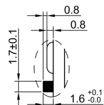
POLARITY PROTECTION DEVICE DETAIL "A" S=2
