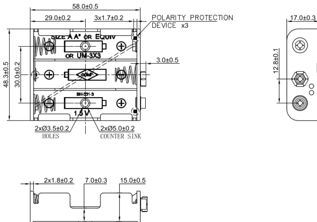
BH-331-3B Shown With Snap Terminals
