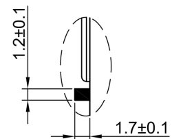
POLARITY PROTECTION DEVICE DETAIL "A" S=2
