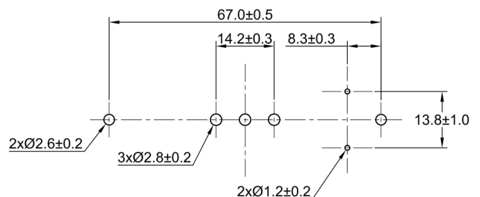
PCB/MOUNTING LAYOUT
