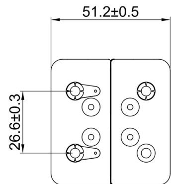
BH-282-1D Shown without solder terminals
