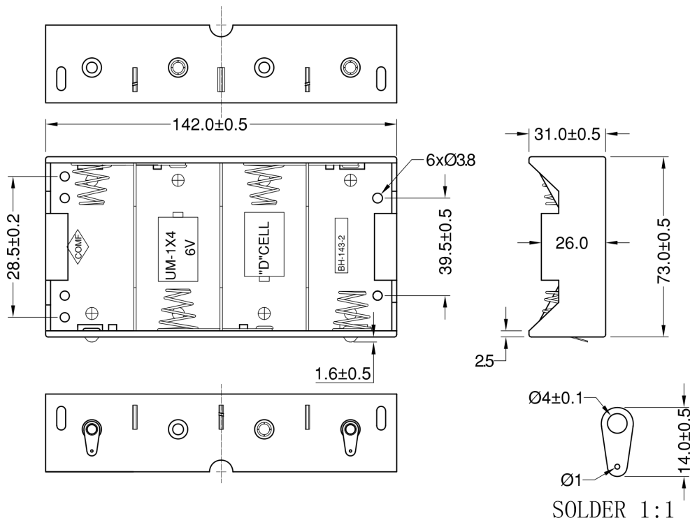
BH-143-2D Shown
