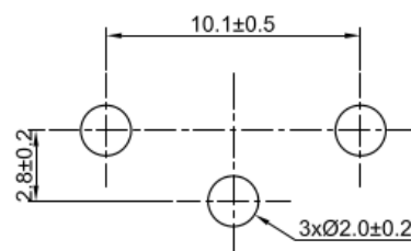
PCB/MOUNTING LAYOUT
