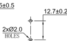
PCB/MOUNTING LAYOUT
