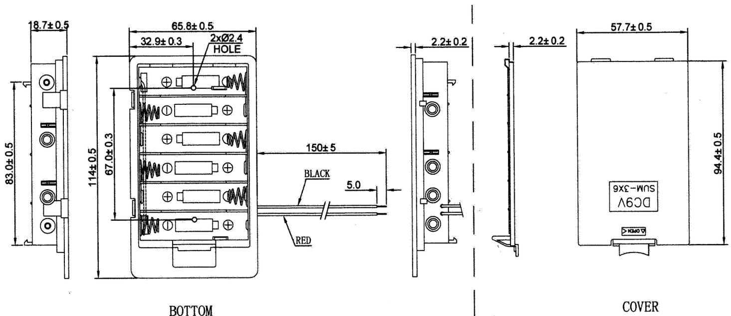
SBH-361A Shown without leads
