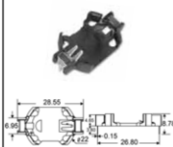
CH016-2032 FOR CR2032
