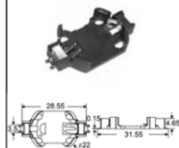
CH017-2032 FOR CR2032
