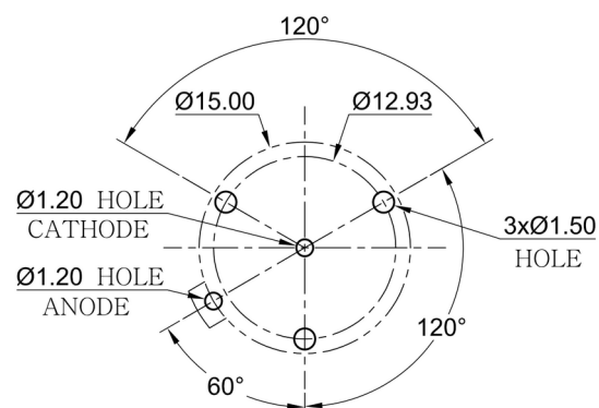
PCB MOUNTING LAYOUT
