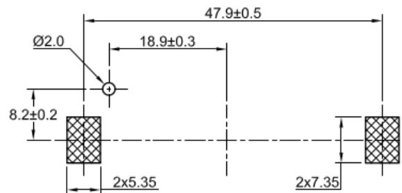
PCB/MOUNTING LAYOUT
