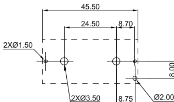
PCB MOUNTING LAYOUT
