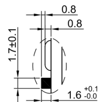
POLARITY PROTECTION DEVICE DETAIL "A" S=2
