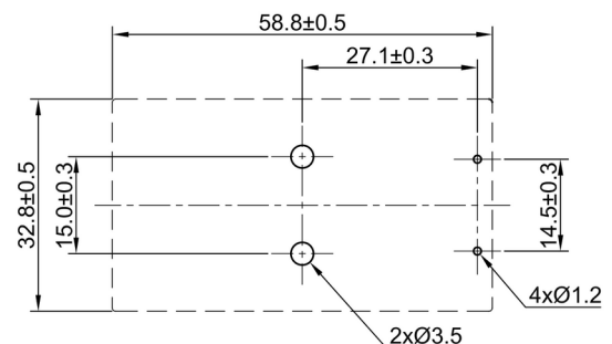
PCB/MOUNTING LAYOUT
