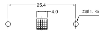
PCB Mounting layout
