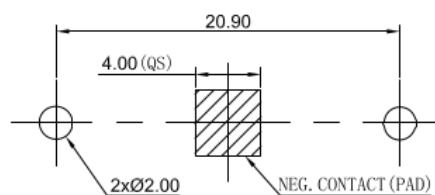
PCB Mounting Layout
