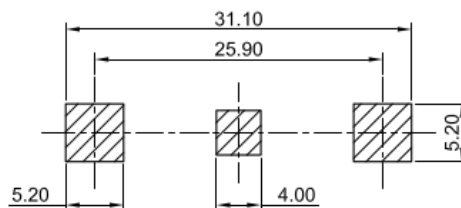
PCB MOUNTING LAYOUT
