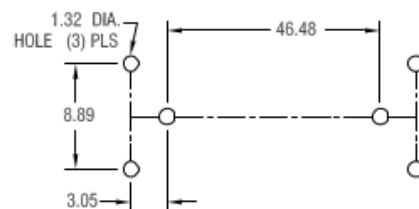
PCB Mounting Layout
