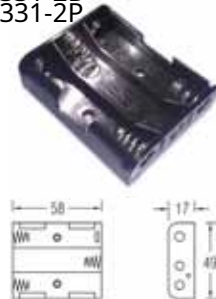
BH331-2A BH331-2B FOR THREE "AA" CELLS BH331-2D BH331-2P
